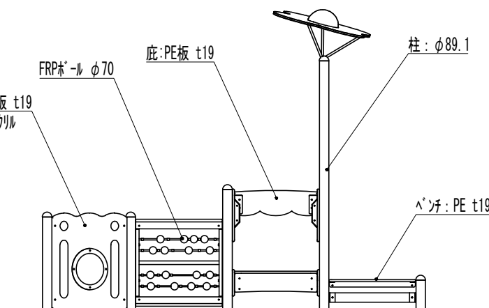
B-B (1:50)
